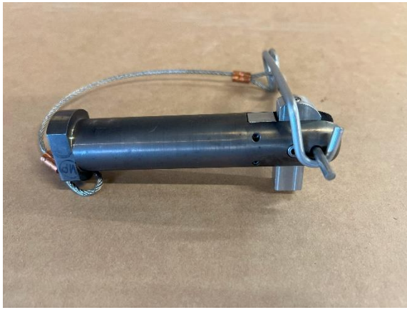
Locking Load Pin Part # LLP-100 Figure 18
