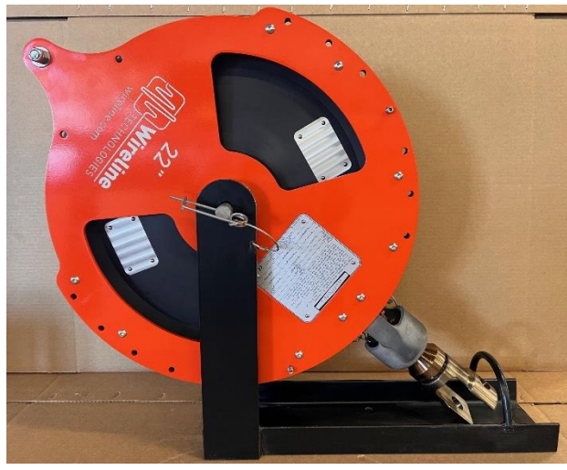
Storage Rack, Part # TS-22-100 Figure 28
