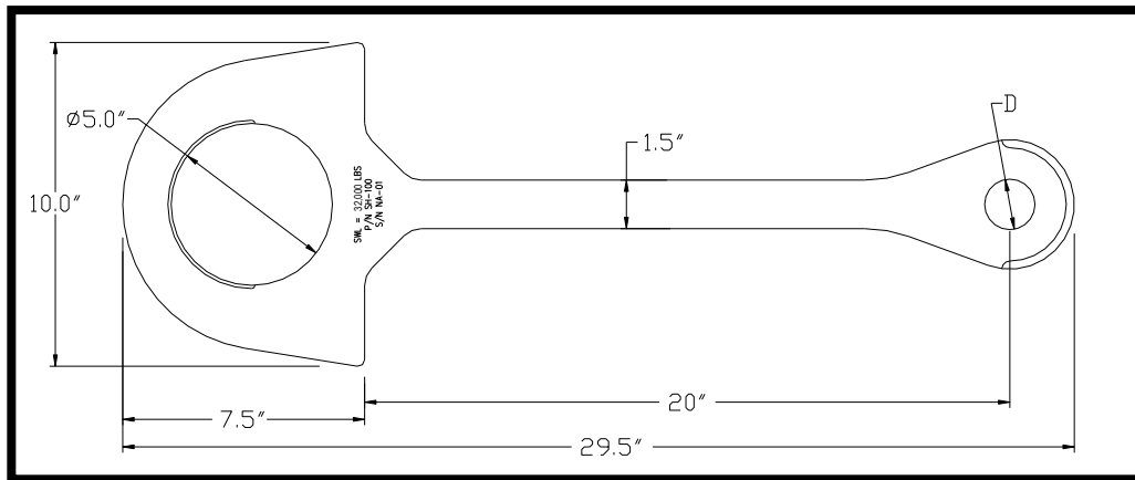
Hanger Bar, Figure 20
