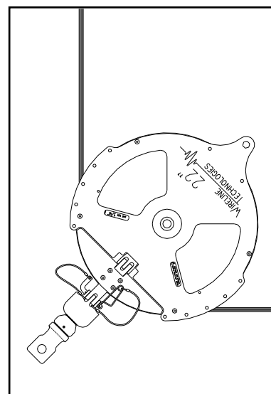
Safe Line Tension for 90-Degree Deflection Figure 4
