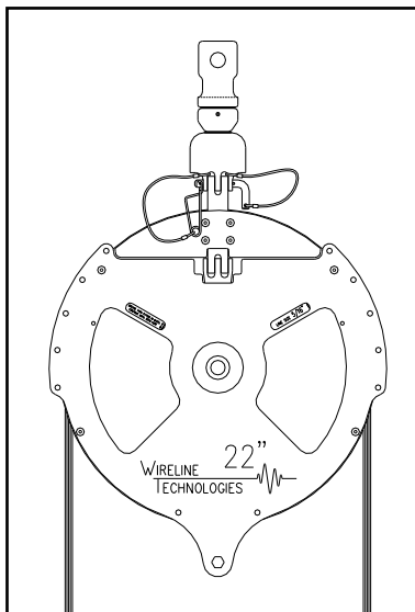
Safe Line Tension for 180-Degree Deflection Figure 3
